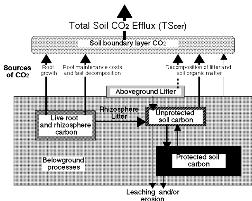
Figure 1. Components of CO 2 efflux from forest soils (TS cer ). TS cer from the soil boundary layer to the atmosphere equals CO 2 production from roots, rhizosphere heterotrophs, litter, and soil heterotrophs when steady state conditions are approached. Abnormal turbulence at the soil surface can produce TS cer which exceeds the rate of CO 2 production by the component processes. The dashed line from the surface litter layer indicates a dynamic process highly dependent on litter water content.
