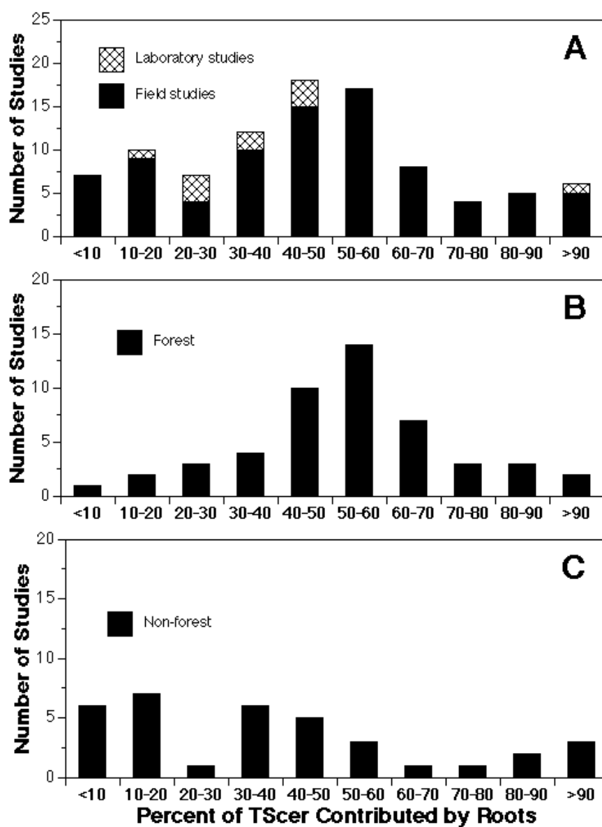
Figure 2. Histograms of the percent root contribution to TS_{cer} for all laboratory and field based studies (A) and separate graphs for forest (B) and nonforest studies (C). The laboratory-based observations were not included in graphs B and C. Measurement periods vary among compiled studies (see Table 1).
